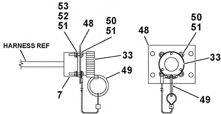
J1939 DIAGNOSTIC CONNECTOR ASSY
